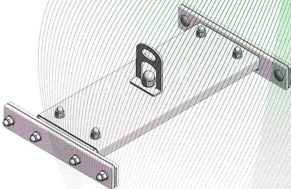
Fig. 1: Anchor device, type: LUX-top® FALZ-PLUS II
